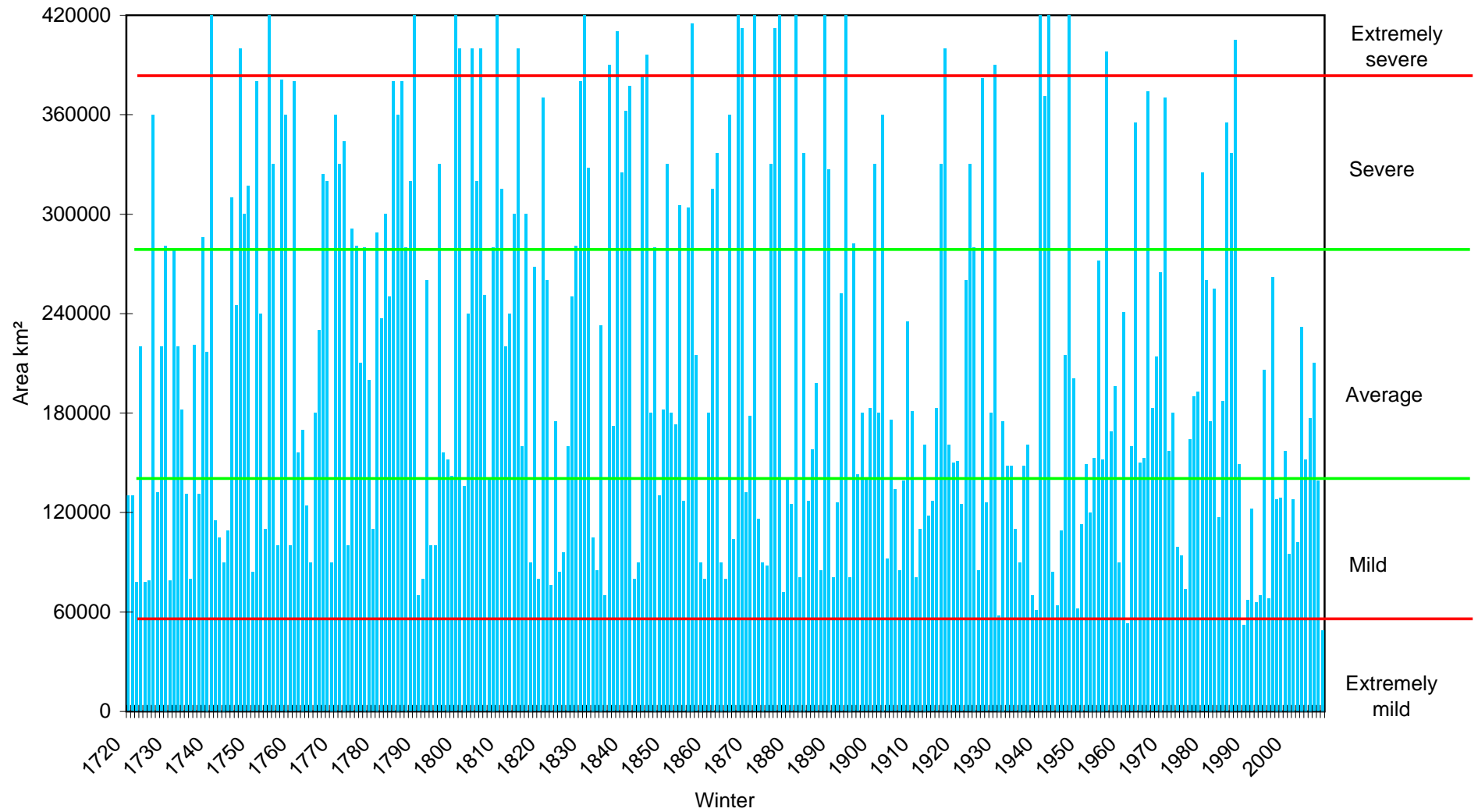
THE MAXIMUM EXTENT OF ICE COVER IN THE BALTIC SEA ON THE WINTERS 1719/20 - 2007/08
